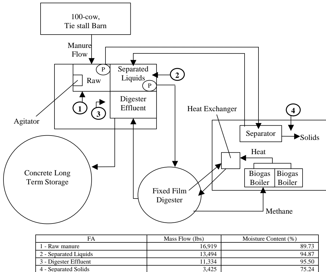
Figure 1. Schematic of Fixed Film Anaerobic Digester System on Farber Dairy Farm.
